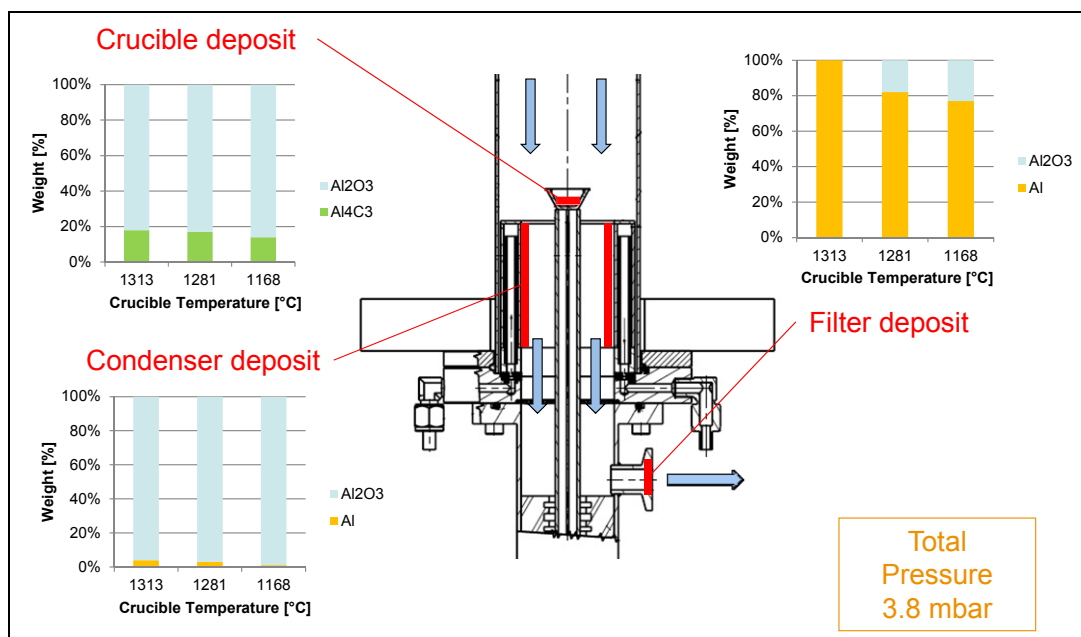
Figure 2: Solar TG experiments in ETHZ for the kinetic modeling of the moderate temperature alumina carbothermic reduction process.
