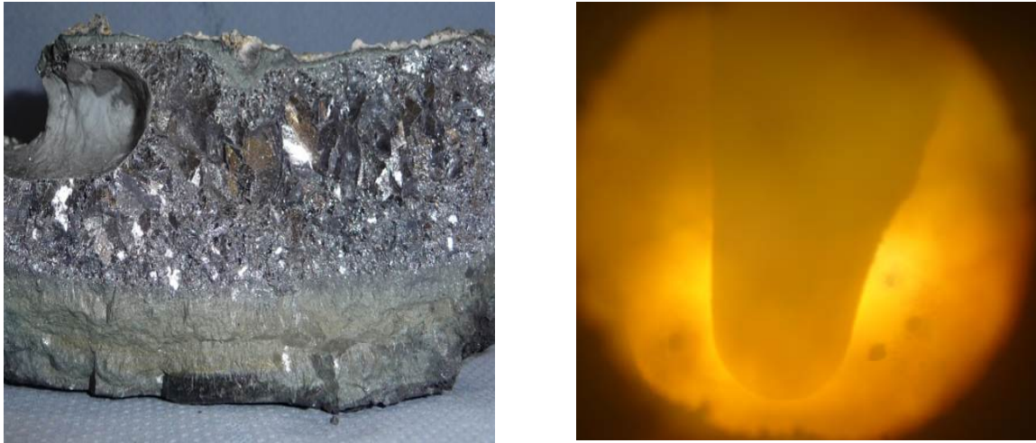
Figure 1 Left: Al-Si alloy phase produced. Right: Gaseous Al production experiment (RWTH-Aachen).
